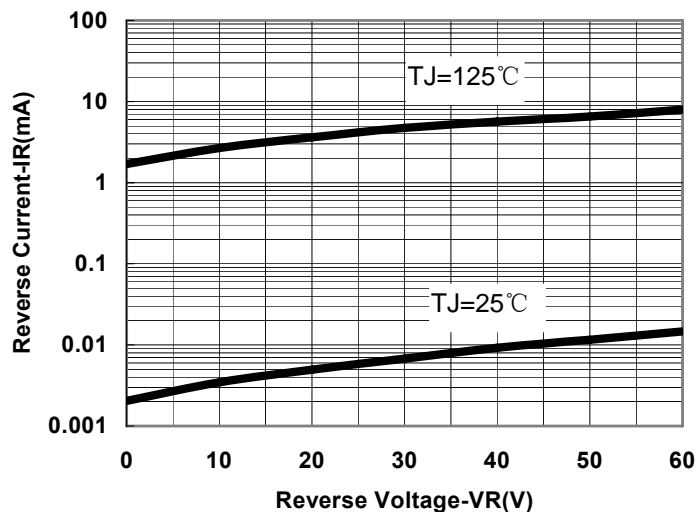
Fig.2-Typical Reverse Characteristics
